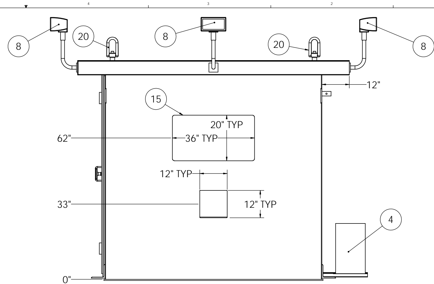
SIDE VIEW (LH AND RH)
