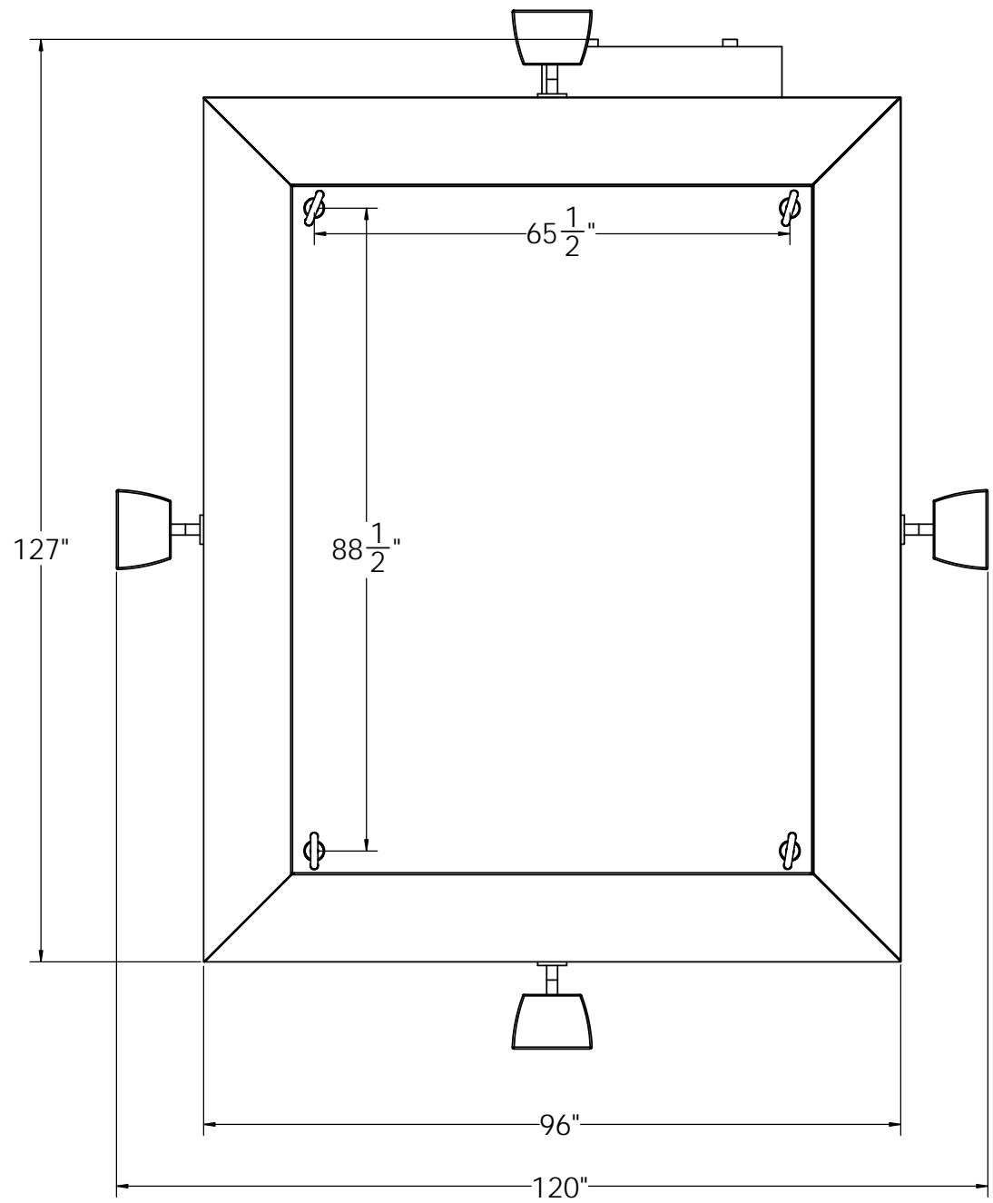
8X6 BRE TOP VIEW AND LIFTER LAYOUT
