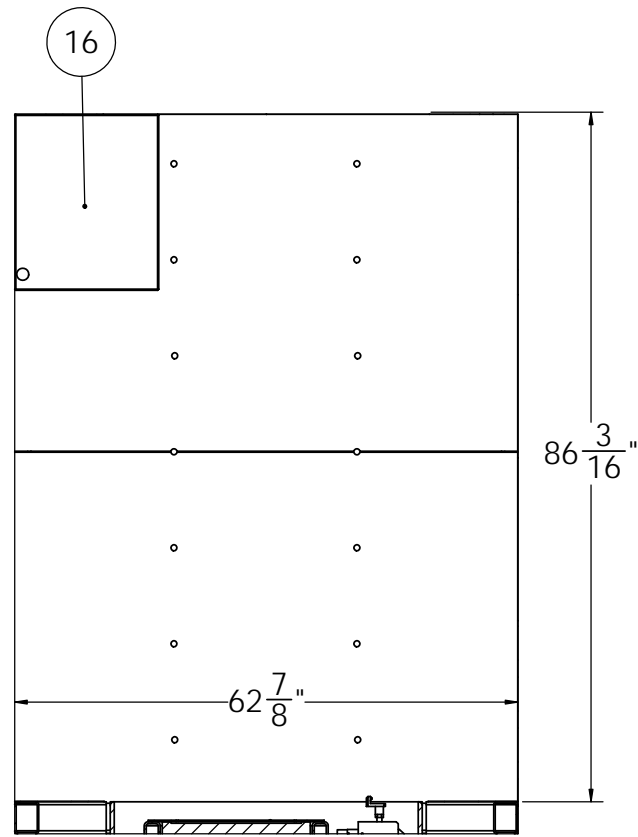
FLOOR PLAN
