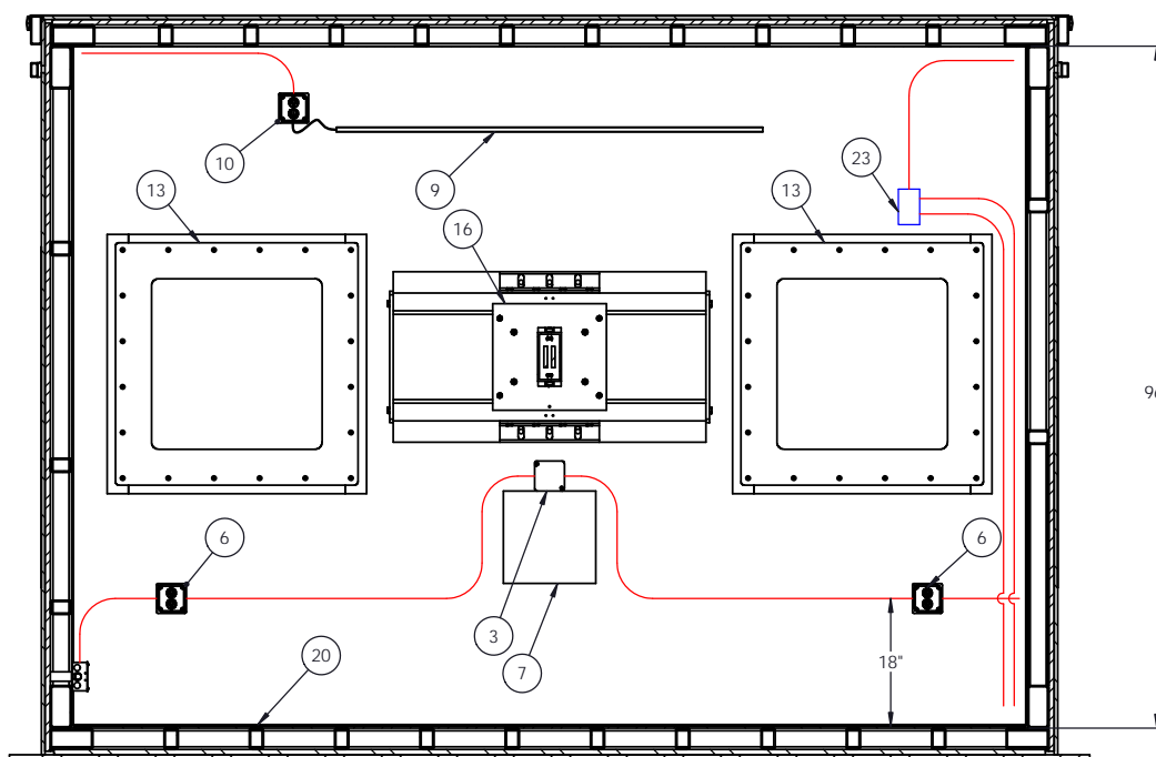
INTERIOR LEFT SIDE ELEVATION
