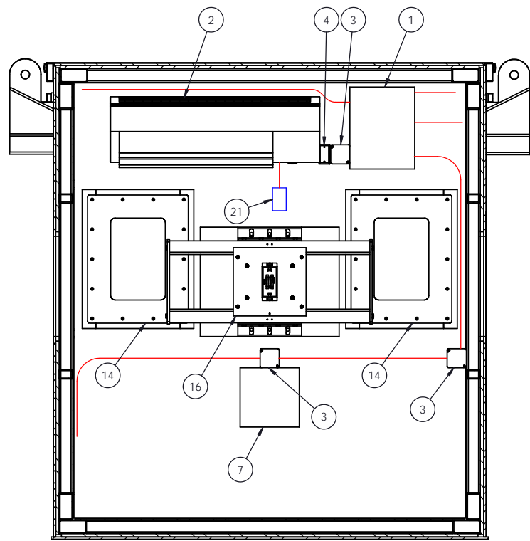
INTERIOR REAR ELEVATION
