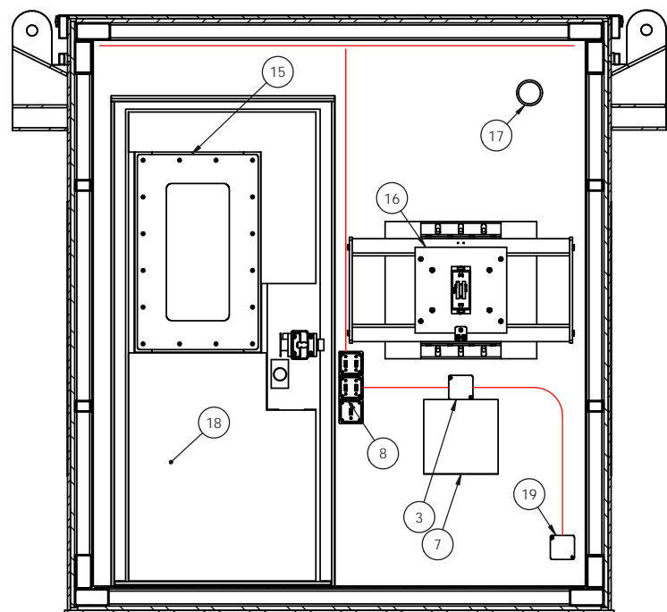
INTERIOR FRONT ELEVATION
