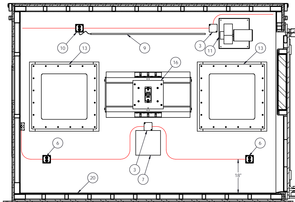
INTERIOR RIGHT SIDE ELEVATION
