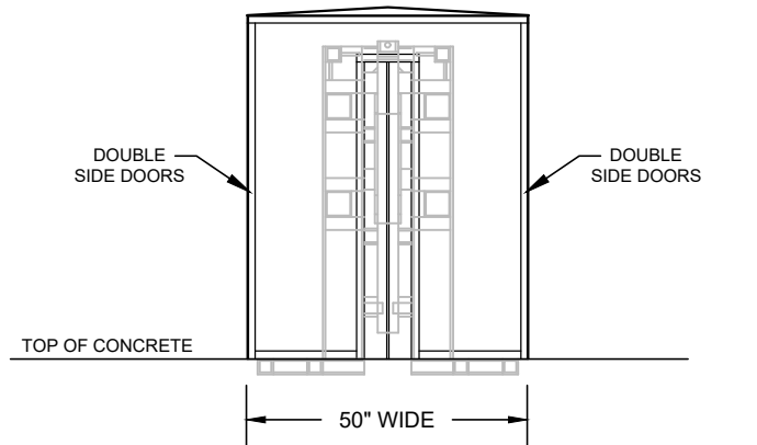
FRONT SIDE
