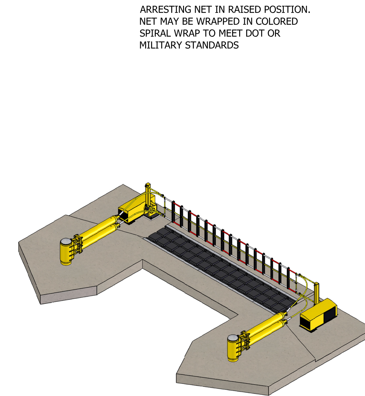
B - ISOMETRIC VIEW SCALE: NTS
