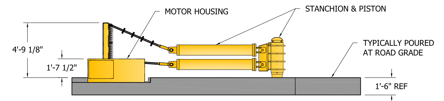
A-2 - SIDE ELEVATION VIEW SCALE: 1/4" = 1'-0"
