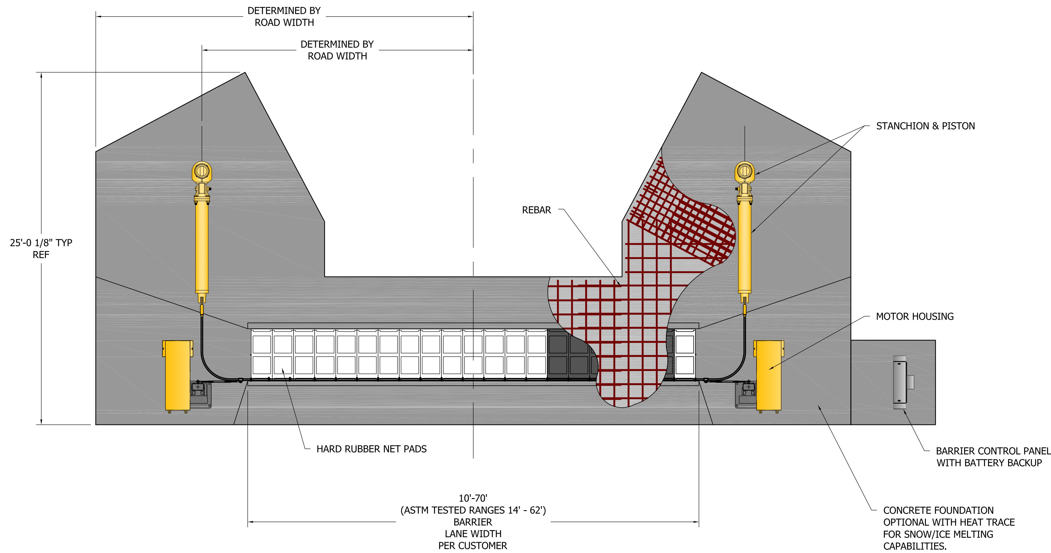
A - PLAN VIEW SCALE: 1/4" = 1'-0"
