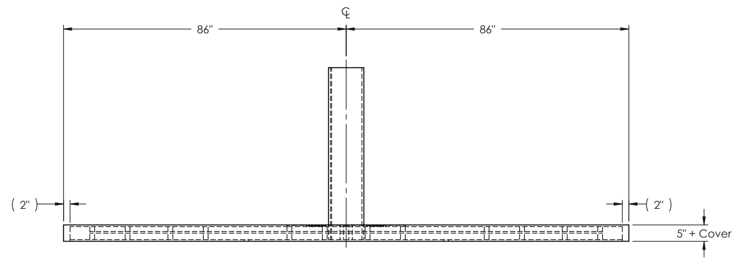
ELEVATION VIEW SCALE 1 : 30
