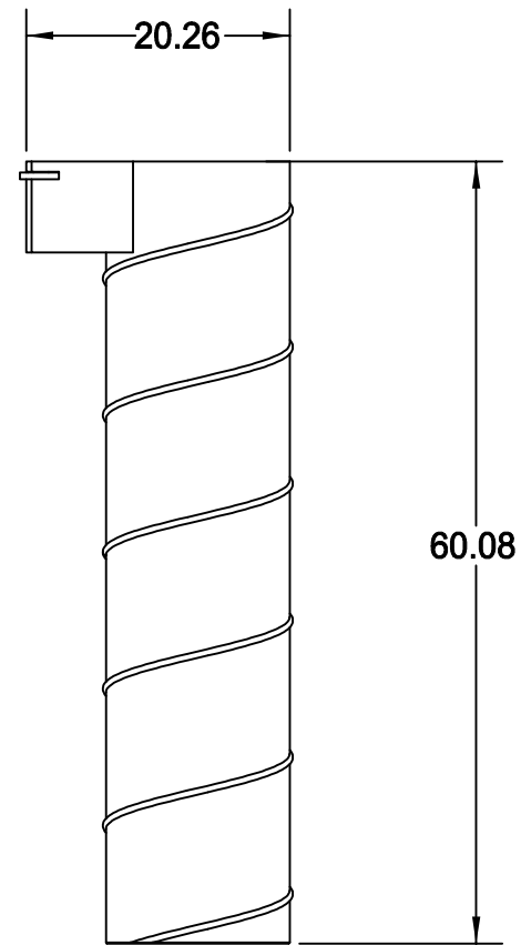
STOWED BOLLARD
