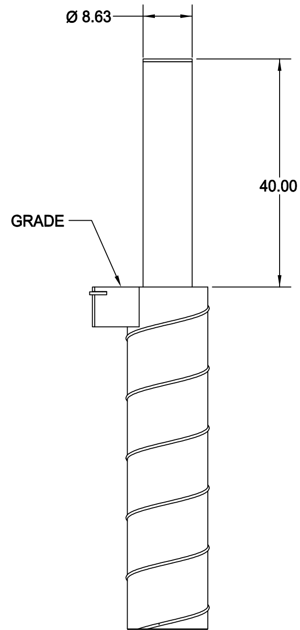
DEPLOYD BOLLARD
