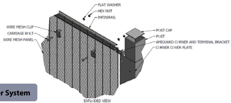
EXPLODED VIEW
