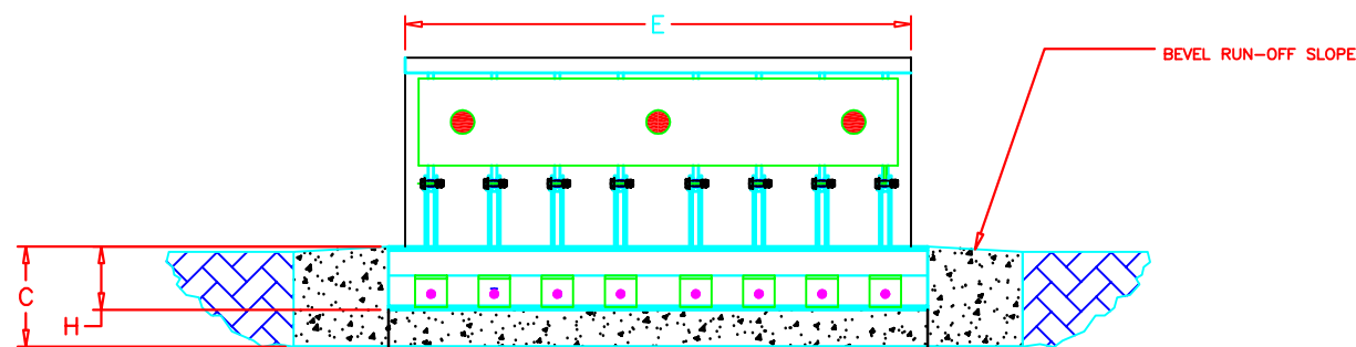
FRONT (ELEVATION) VIEW
