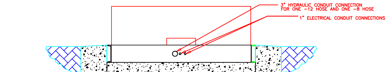
BACK (ELEVATION) VIEW
