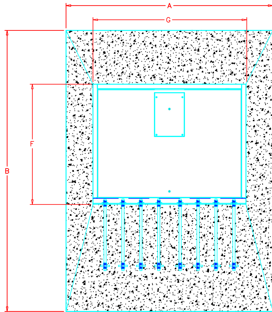
TOP (PLAN) VIEW
