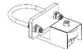
SINGLE WHEEL GUIDE W/ROUND U-BOLTS
