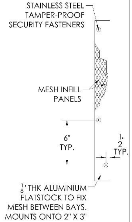
MESH PANEL MOUNT DETAIL SCALE: 1-1/2" = 1'
